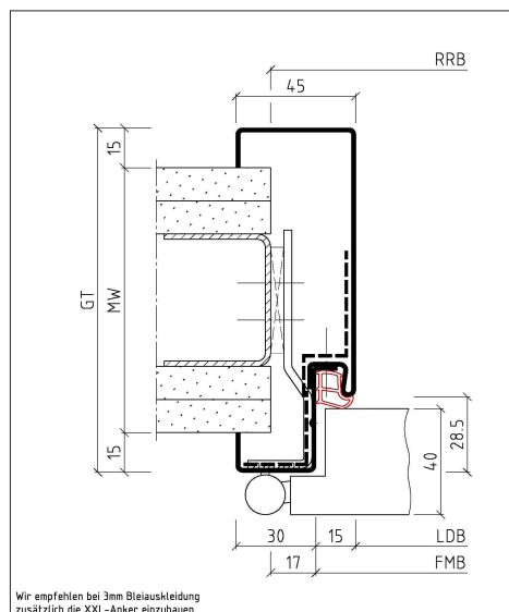
2-schalige Zarge
